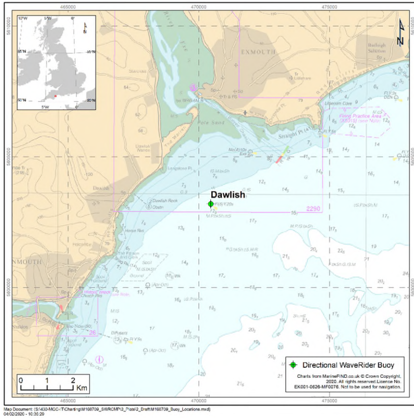
Figure 1: Dawlish Wave Buoy
